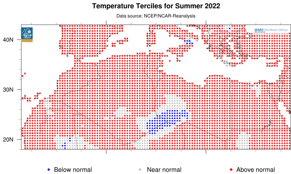
Figure 18: Tercile distribution for temperature of JJA 2022 in North Africa, reference period 1981-2010. Source: INM, Data from NCEP/NCAR reanalysis, http://www.esrl.noaa.gov
