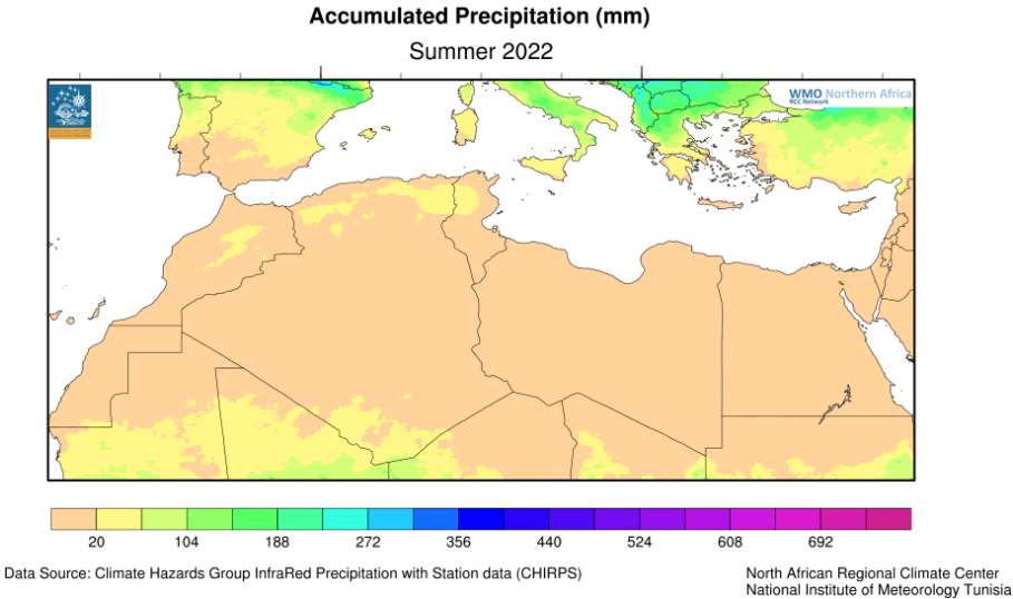
Figure 22: Total precipitation for summer season 2022 in North Africa (in mm). Source: INM, Data from CHIRPS: ftp://ftp.chc.ucsb.edu/
