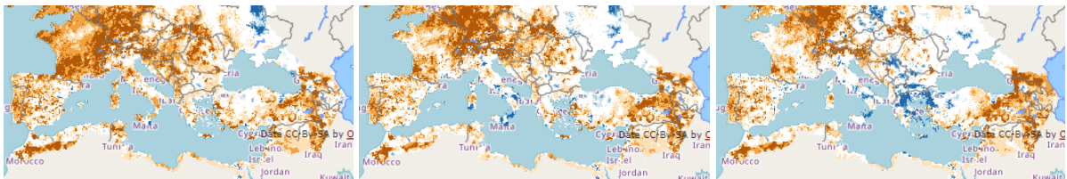
Figure 11: Soil moisture anomalies for 10-day periods in summer 2022 (brown: below normal, blue: above normal, 1995-2021 reference). Source: European Drought Observatory (EDO), https://edo.jrc.ec.europa.eu/edov2/php/index.php?id=1138
