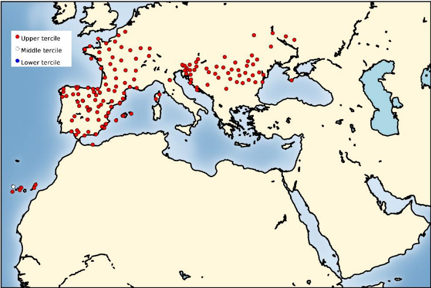
TEMPERATURE JJA 2022 (ECA&D data) (reference period 1981-2010)
