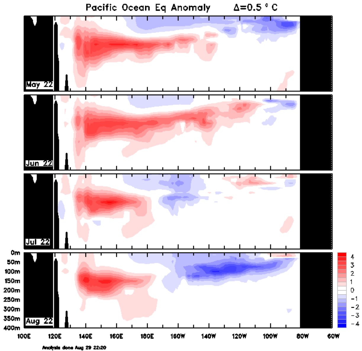
Figure 3: 4-month sequence of vertical temperature anomaly sections at the equatorial Pacific for May-August 2022. Source: Australian Government, Bureau of Meteorology (BOM), http://www.bom.gov.au/cgi-bin/oceanography/wrap_ocean_analysis.pl?id=IDYOC007&year=2022&month=08
